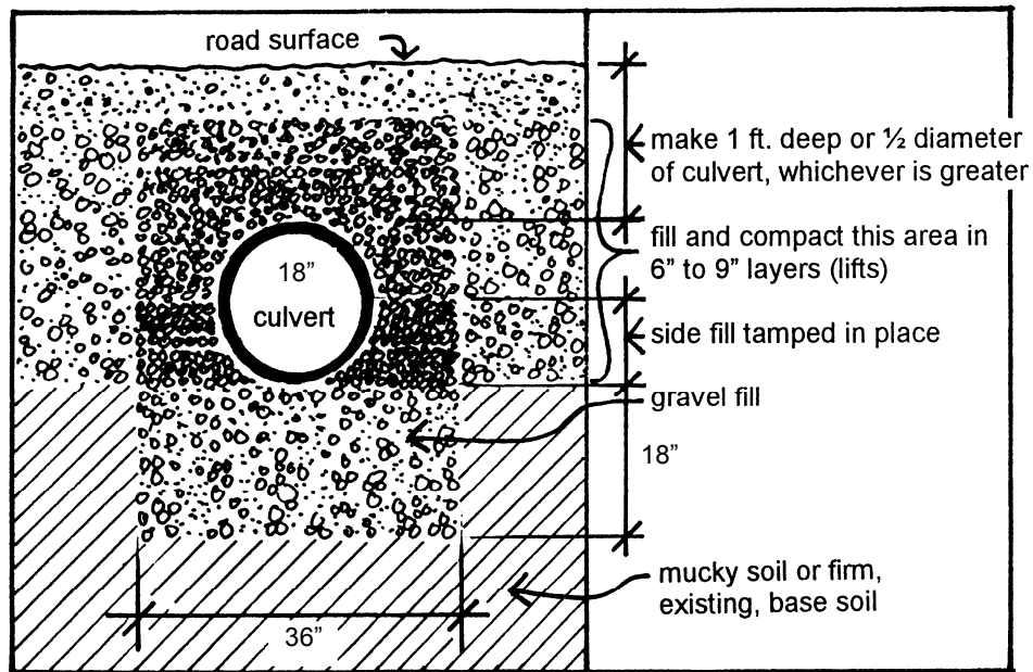
Figure 30. Culvert Installation
